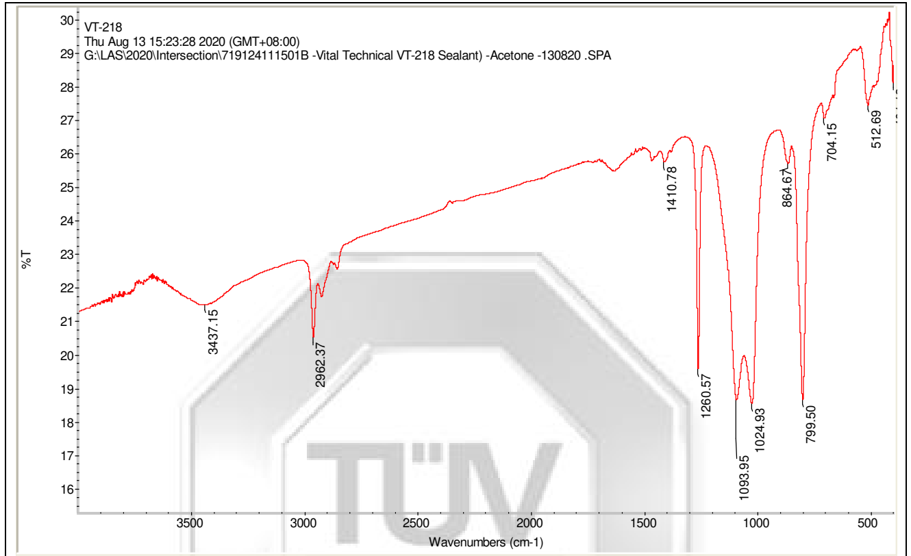
Figure 1: Infrared Spectrum of 'AS-208' Glass & Metal Sealant
